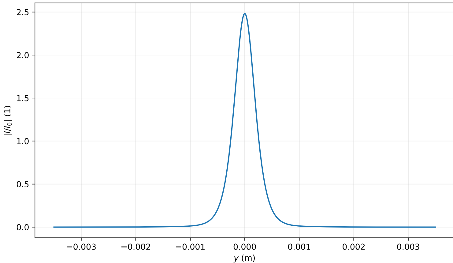
Intensity profile I(x=0, y, z=2.707)/I_0 , \text{Pin}=1.0\text{Pcr} , artificial time
